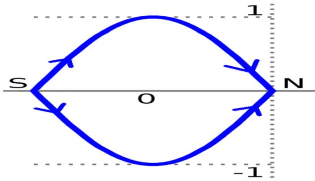
Illustration 2.18: Closed Sine Wave
