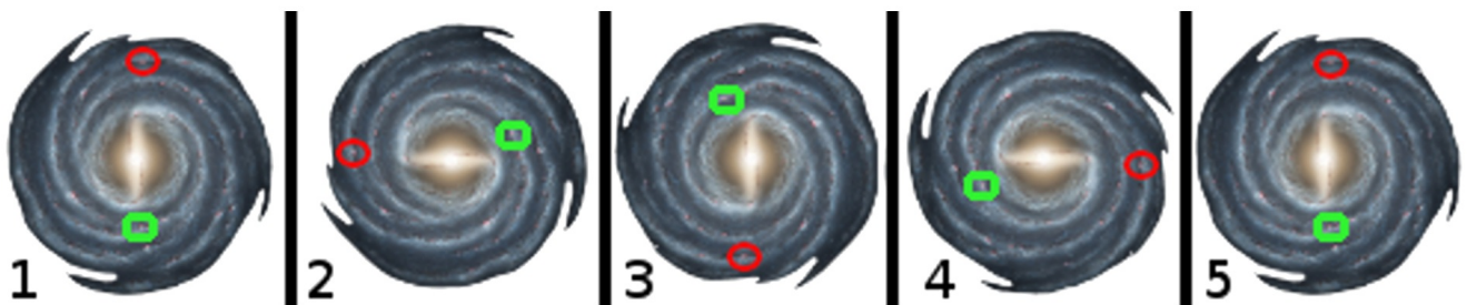
Illustration: The Galaxy Spinning all Solar Systems at the same Rate
