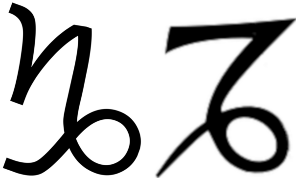
Illustration 4.39: Ancient to New Capricorn Sign
