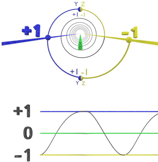
Illustration 4.31: Trinary Electron/Engine Orbital Path - Trinary Helix (3D and 2D)
