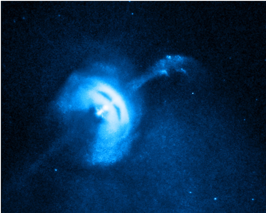
Illustration 4.29: Vela Pulsar
