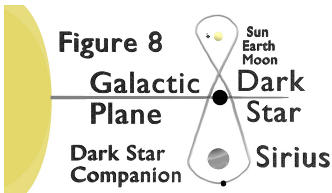
Illustration 4.28: Dark Stars Figure 8
