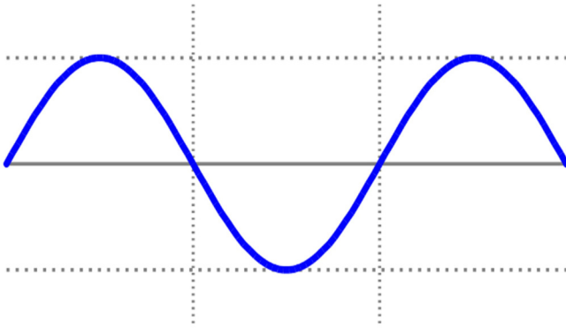
Sine Wave
