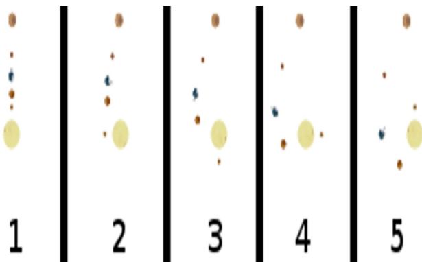
Illustration 3.03: The Sun Spinning all Planets in it is System at different Rates
