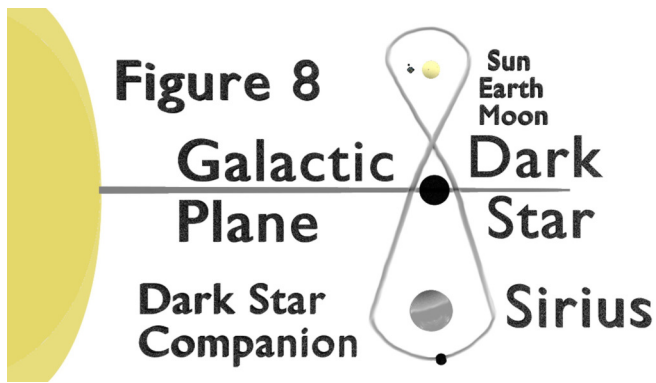
Illustration 4.03: Solar System path with Dark Star
