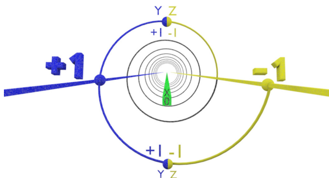
Illustration 2.22: An Electron Orbital Path around a Magnet
