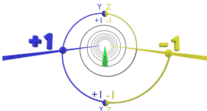
Illustration 4.20: Trinary Atom Waveform
