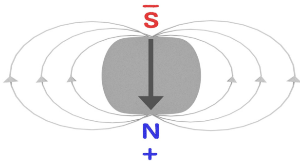
Illustration 4.15: Trinary Energy Flow does not show
