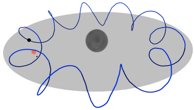
Illustration A2: Complete Orbital path of Sun around Galaxy
