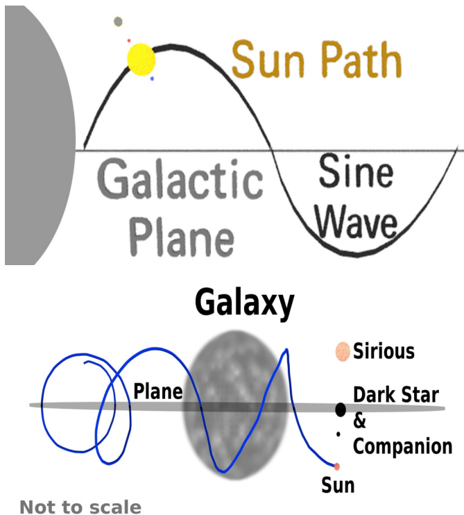
Illustration 3.07: Sun Path makes Sine Wave and Helix Illustration 3.08: Sun Path makes Sine Wave and Helix
