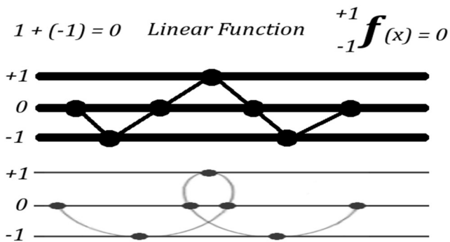
Illustration 4.33: Trinary Mathematical Formula
