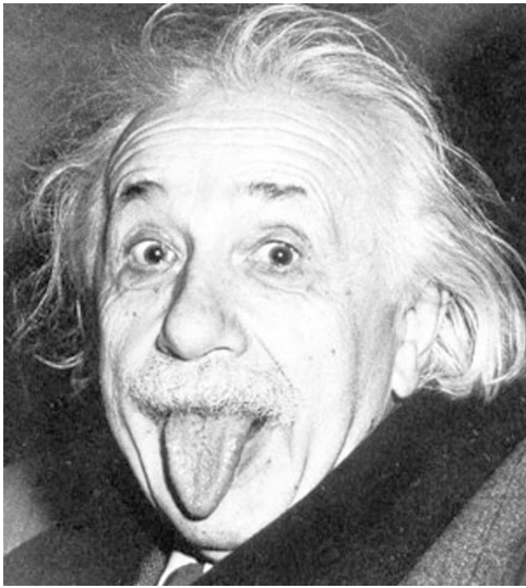
Illustration 4.12: Albert Einstein's impression of General Relativity
