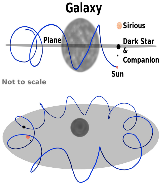
Illustration 4.35: Complete Orbital path of Sun around Galaxy
