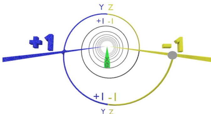
Illustration 2.03: Atom (-1) State [1]
