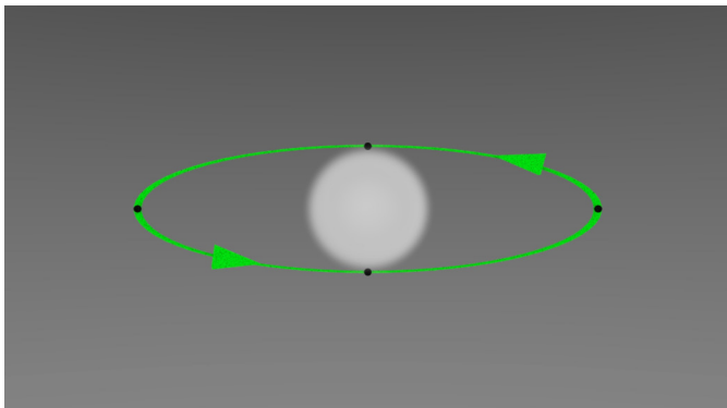
Illustration 4.23: Galaxy's Dark Stars
