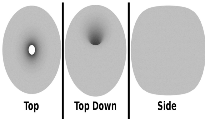
Illustration 4.14: Trinary Universe Sphere
