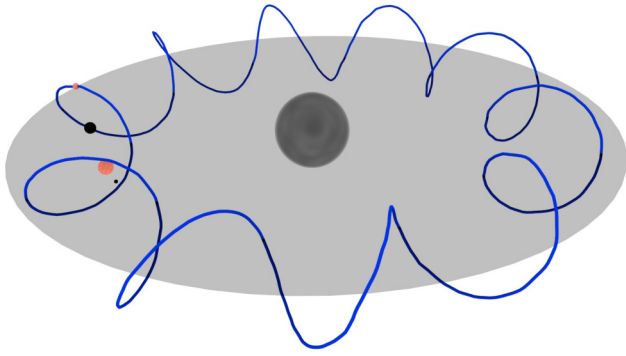
Illustration 4.07: Orbital path of Sun around Galaxy one complete Orbit
