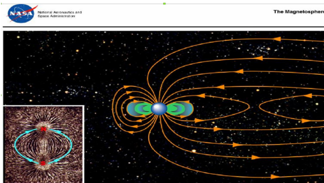
Magnetosphere
