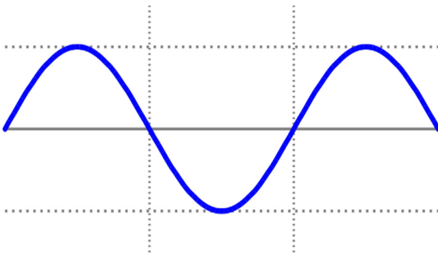
Illustration 2.16: Sine Wave
