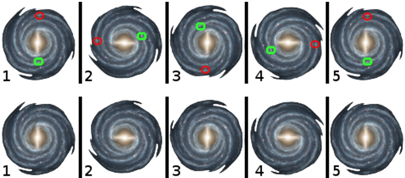
The Galaxy Spinning all Solar Systems at the same Rate but not speed
