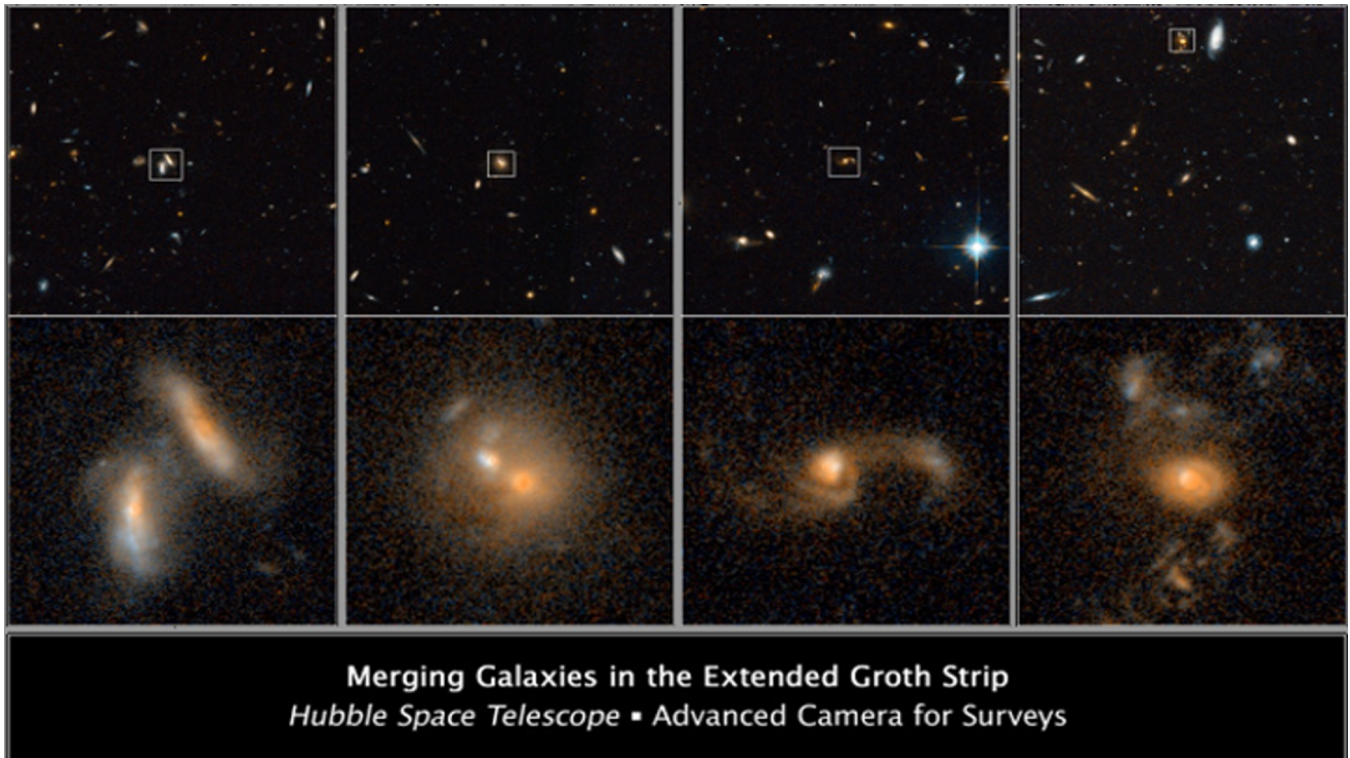
Illustration 4.11: Merging Galaxies
