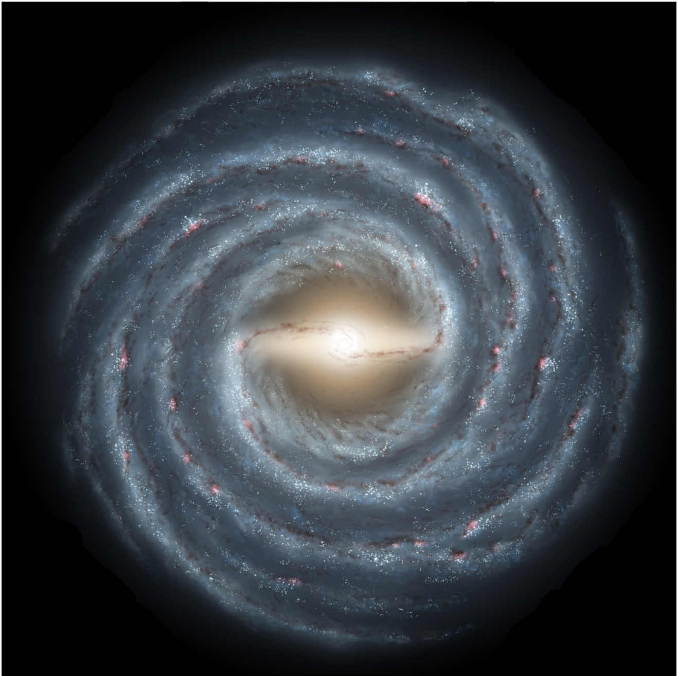
Illustration 4.09: Typical Barred Galaxy
