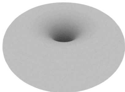
Illustration 2.01: Hydrogen Atom
