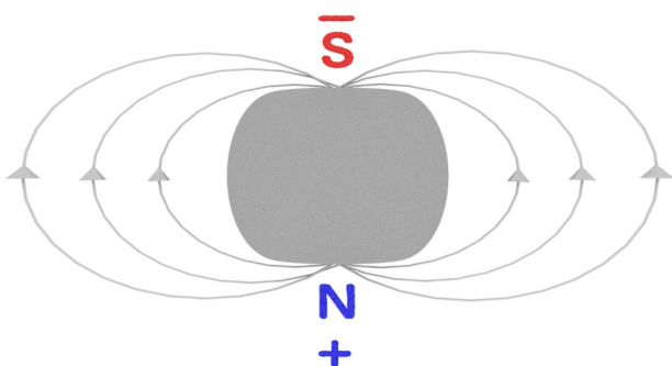
Illustration 2.19: Magnetic Poles of an Atom
