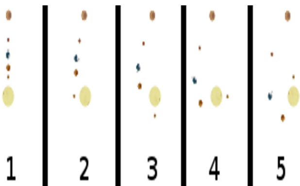
Illustration 4.01: The Sun Spinning all Planets in its System at different Rates
