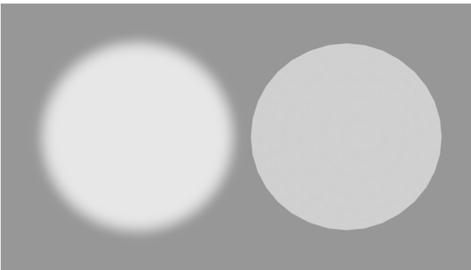
Illustration 2.27: Creation of an Atom: Step 2 - Atom
