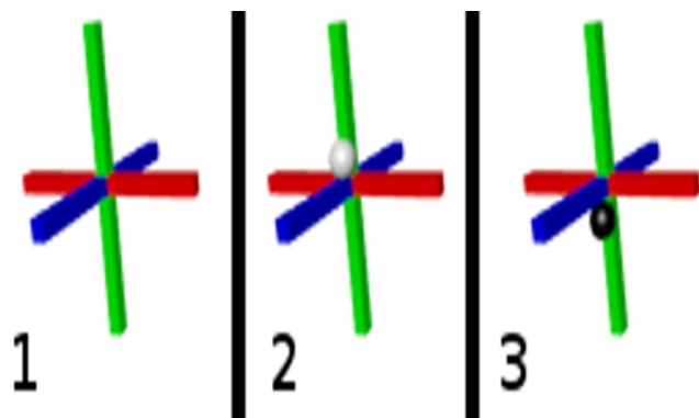
Illustration 2.07: Trinary Energy shown with all 3 States
