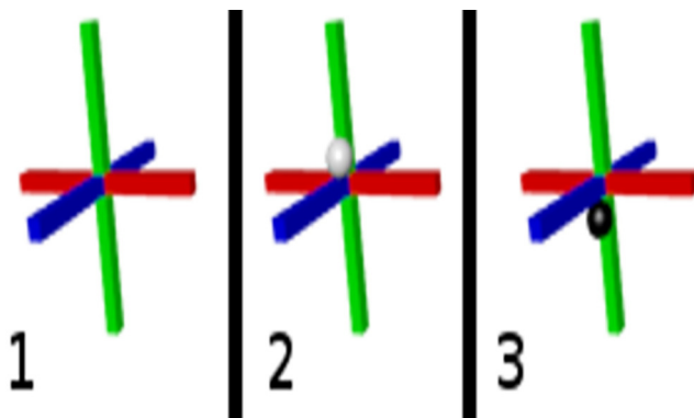
Illustration 2.25: Vertex of Photon, Atom or Trinary Energy
