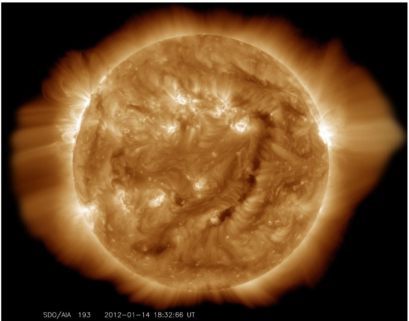
Illustration 3.01: The Sun
