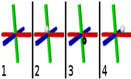
ILLustration 2.06: Vertice Matrix shows Static Light moving
