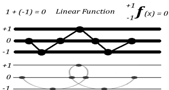
Illustration 4.16: Trinary Mathematical Formula
