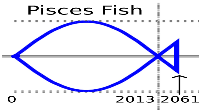
Illustration 4.36: Pisces the Fish Waveform
