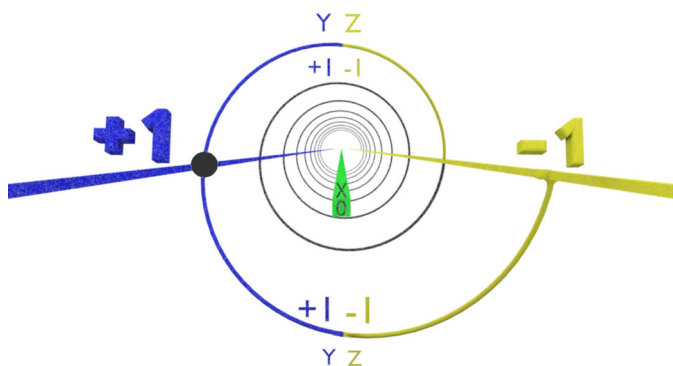
Illustration 2.02: Atom ( \pm 1 ) State [1]
