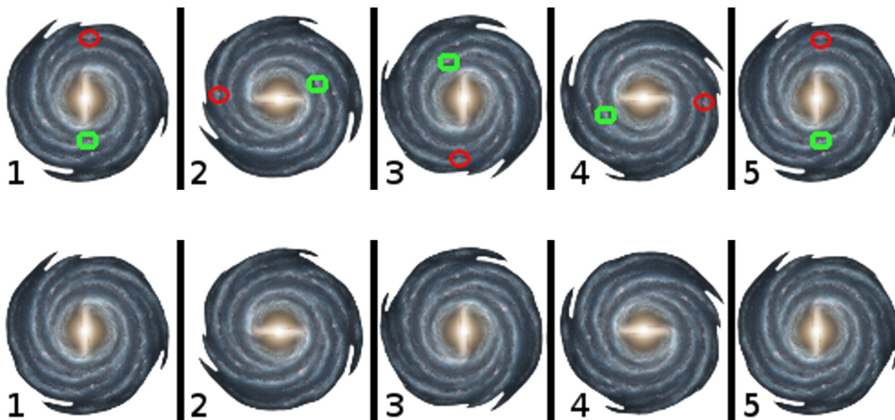
Illustration 4.27: The Galaxy Spinning all Solar Systems at the same Time
