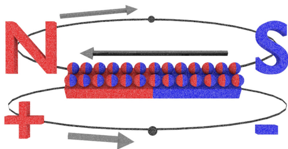
Illustration 2.21: Magnet with extra Electrons
