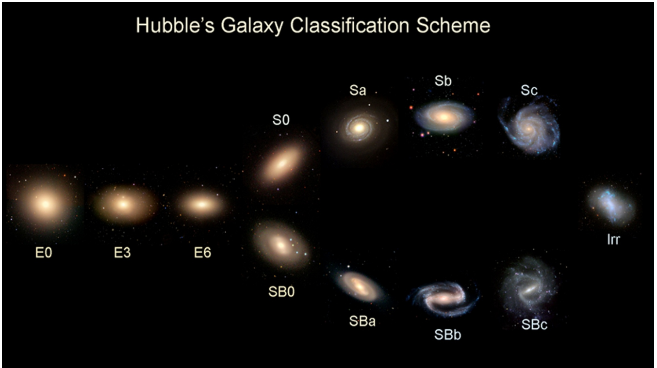
Illustration 4.10: Hubble's Galaxy Classification
