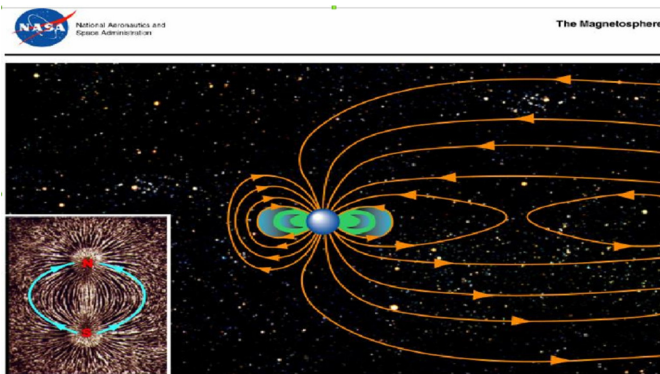
Illustration 2.17: Magnetosphere
