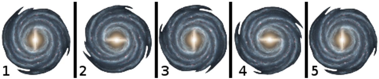
Illustration 4.02: The Galaxy Spinning all Solar Systems at the same Rate
