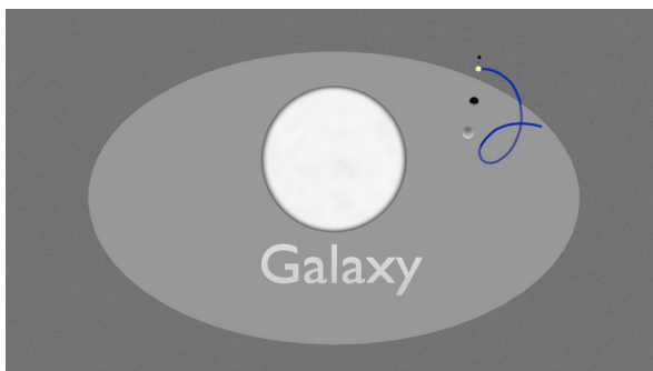
Illustration 2.2: Sun Path makes Sine Wave and Helix Full Size
