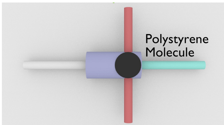
Illustration 9.4: Polystyrene Molecule Full Size
